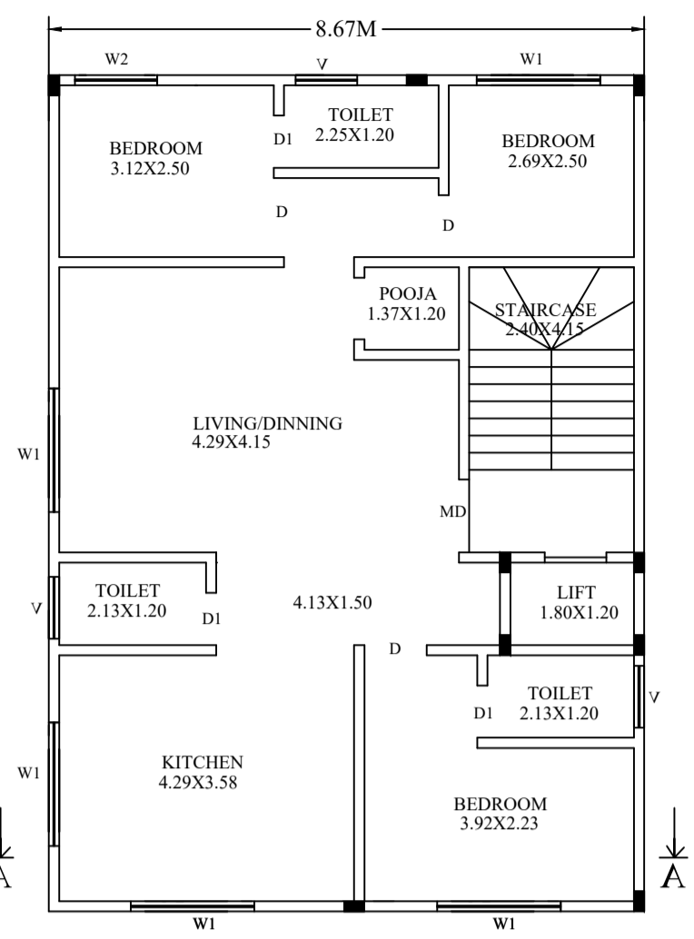
TYP:GROUND & FIRST FLOOR PLAN
